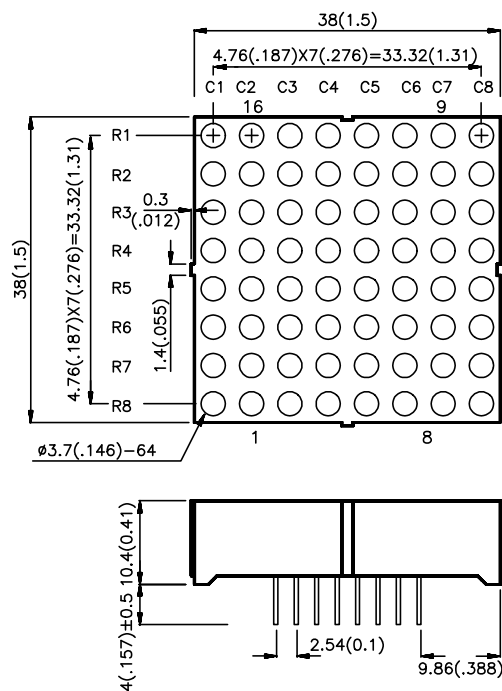
Package Dimensions
